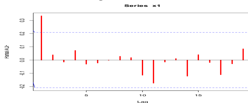
Figure 4: PACF of x_1
