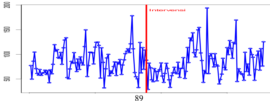
Figure 1: Plot of time series data and Intervention
