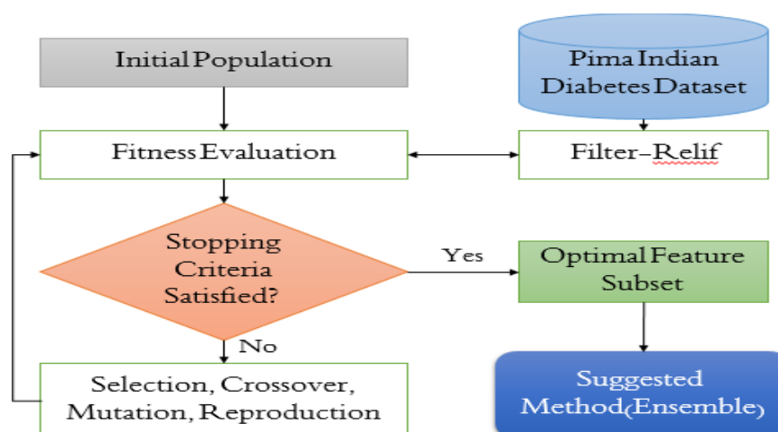
Fig. 2: Proposed flowchart of the hybrid method
