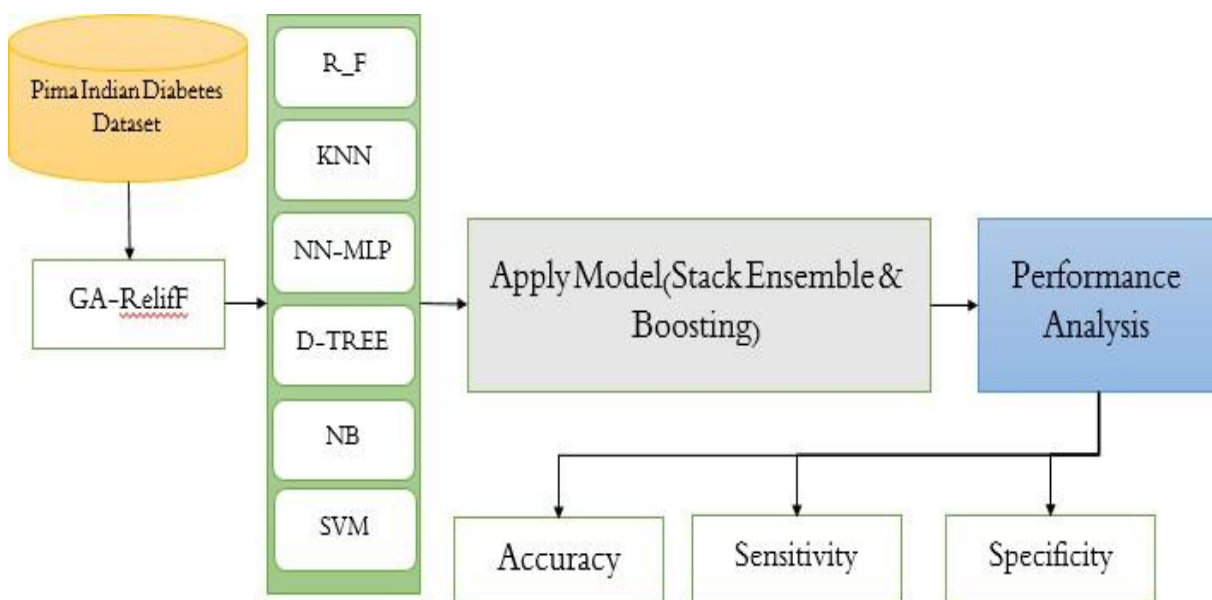
Fig.1: Shows our proposed flowchart
